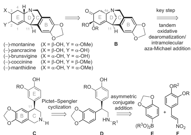
Scheme 4. Retrosynthetic analysis.
